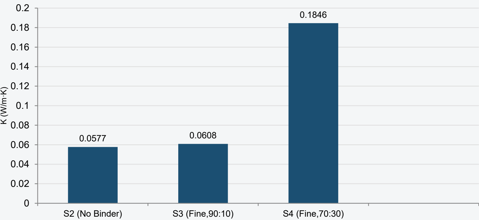
Fig. 18: Thermal Conductivity vs. ASTM C168 Threshold
